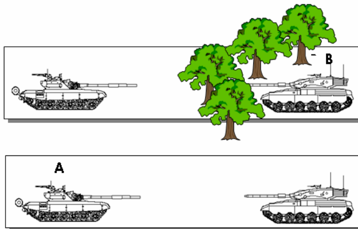
Figure 6: Terrain Miscorrelation.
